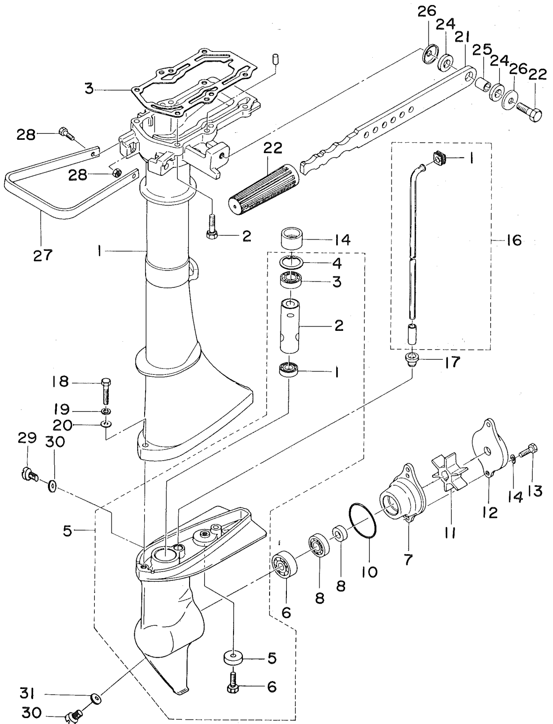
Fig. 6-A DRIVE SHAFT HOUSING, GEAR CASE & STEERING HANDLE
