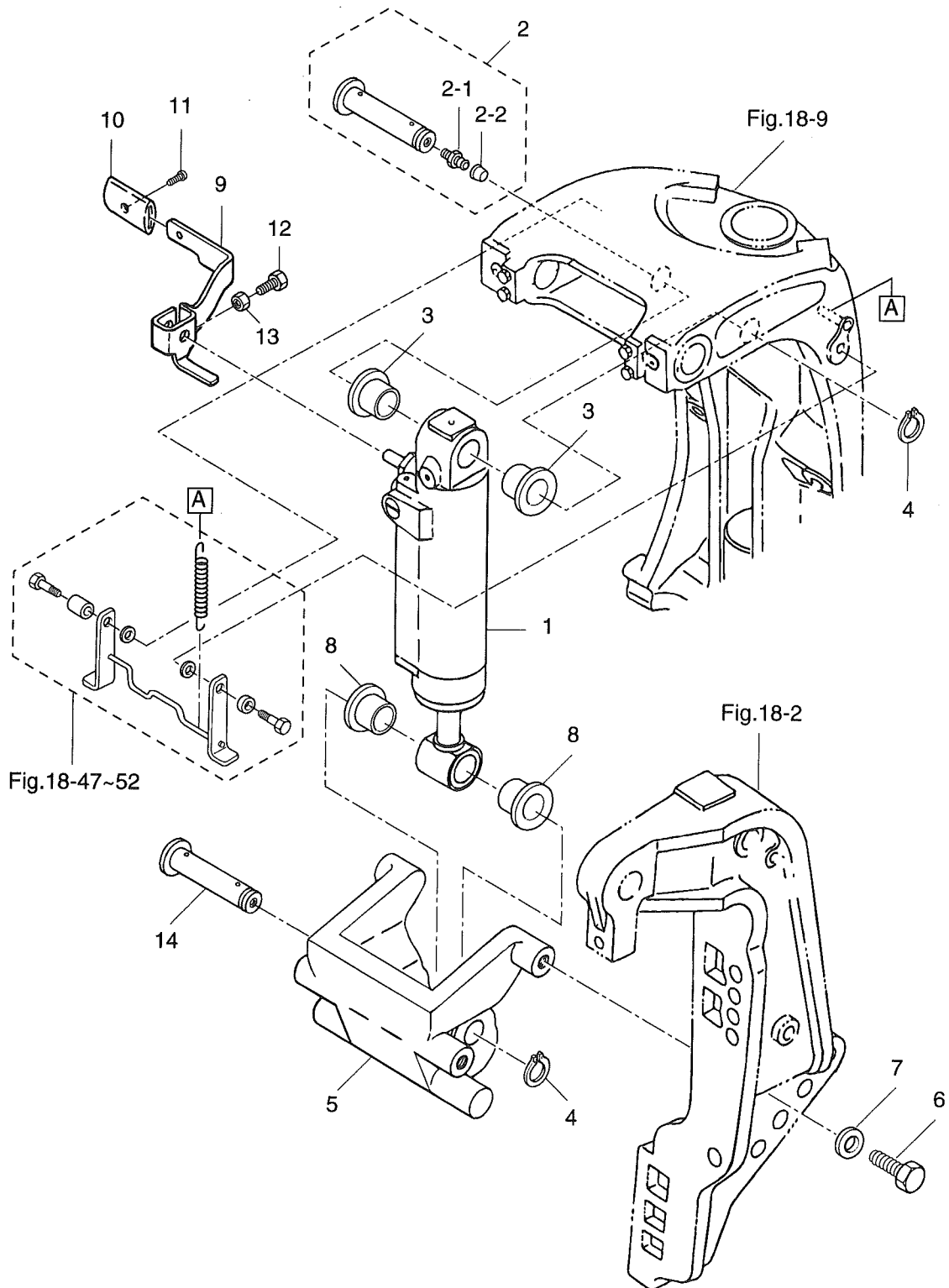
Fig. 21 GAS ASSIST MANUAL TILT (for G Type)
