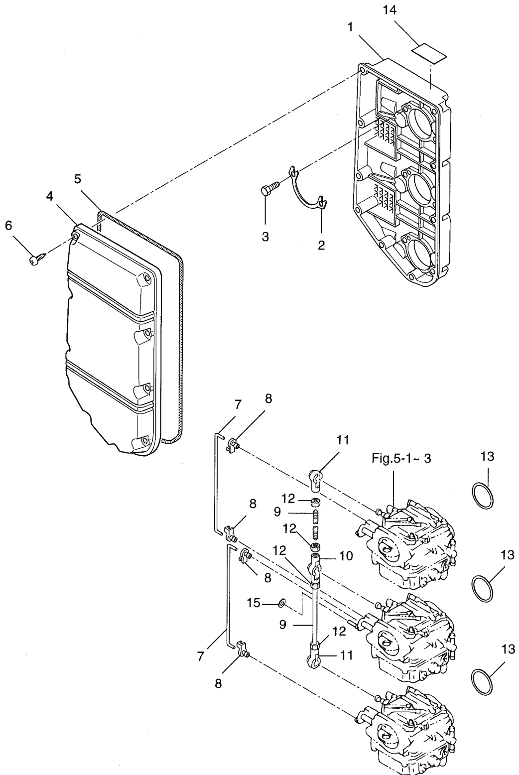
Fig. 4 AIR SILENCER
