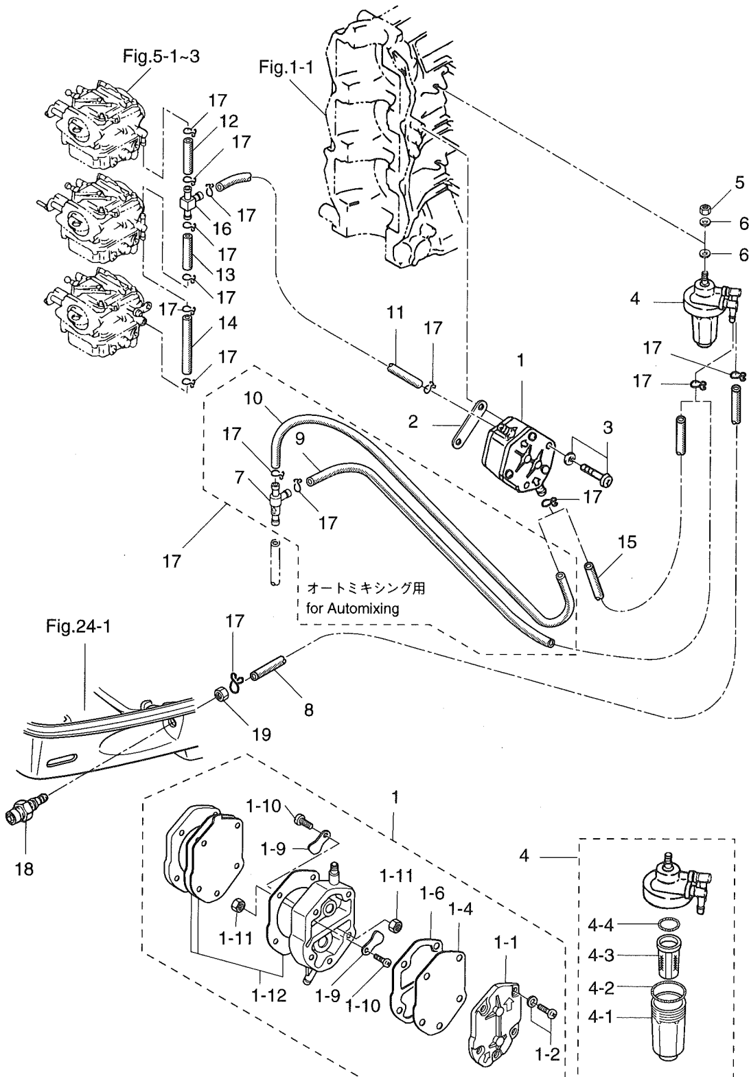
Fig. 6 FUEL LINE
